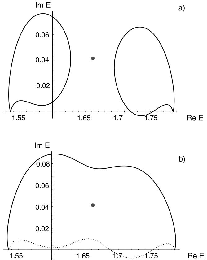
Fig. 2. Contours in the complex energy plane. The top illustrates contours for each level, if a closed loop is described in the \lambda -plane without encircling the exceptional point. The bottom illustrates the energy contour produced by two (equal) closed loops in the \lambda -plane, which encircle the exceptional point. The solid line corresponds to the first closed loop in the \lambda -plane and the dotted line to the subsequent loop. The solid dot is the position where the contours would meet, if the loops crossed the exceptional point in the \lambda -plane.
